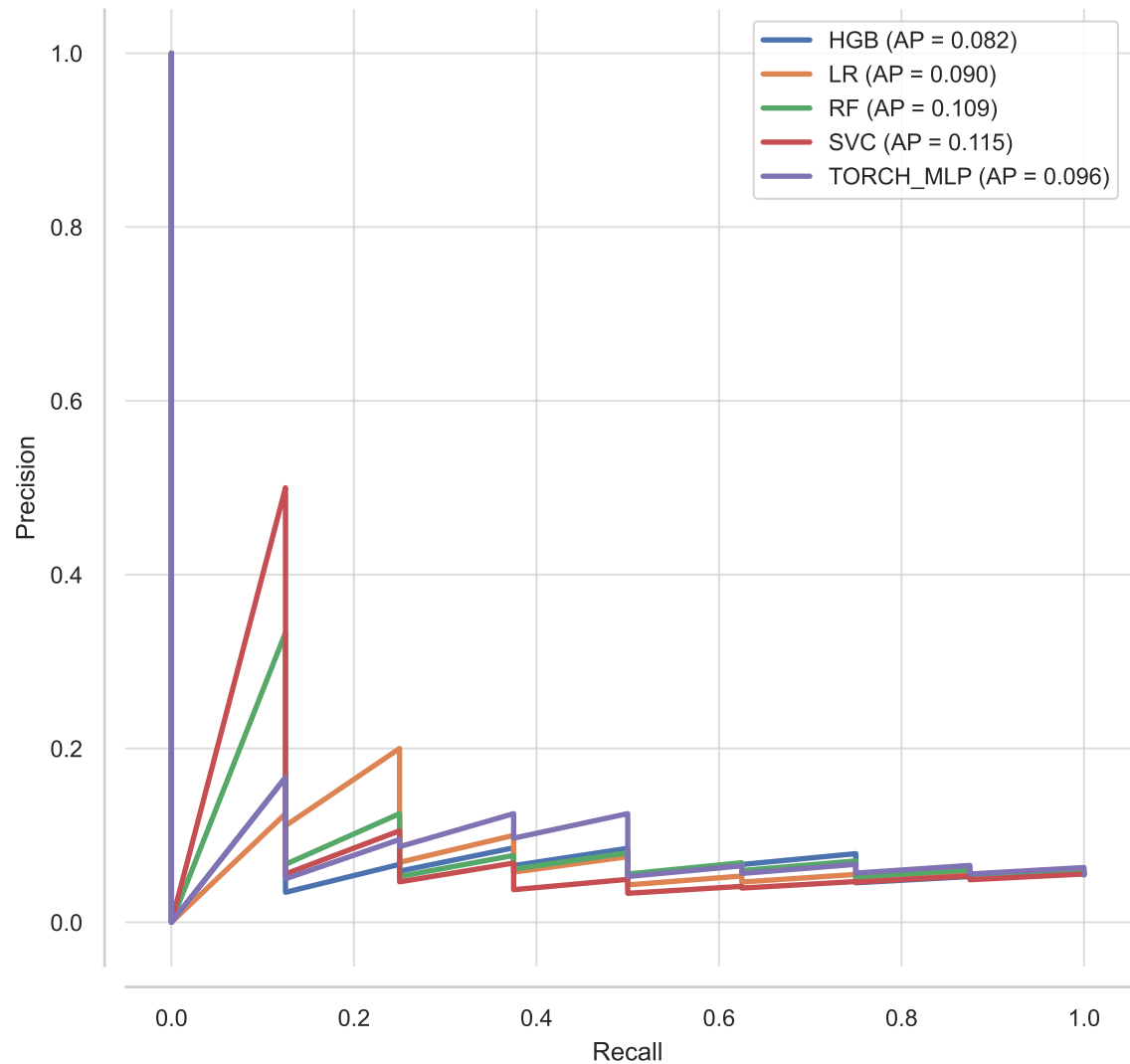
Combined PR Curve (Severe complication)
